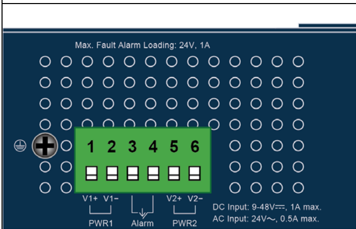
Figure 2-1-3: IGS-4215-16T2S Top View
