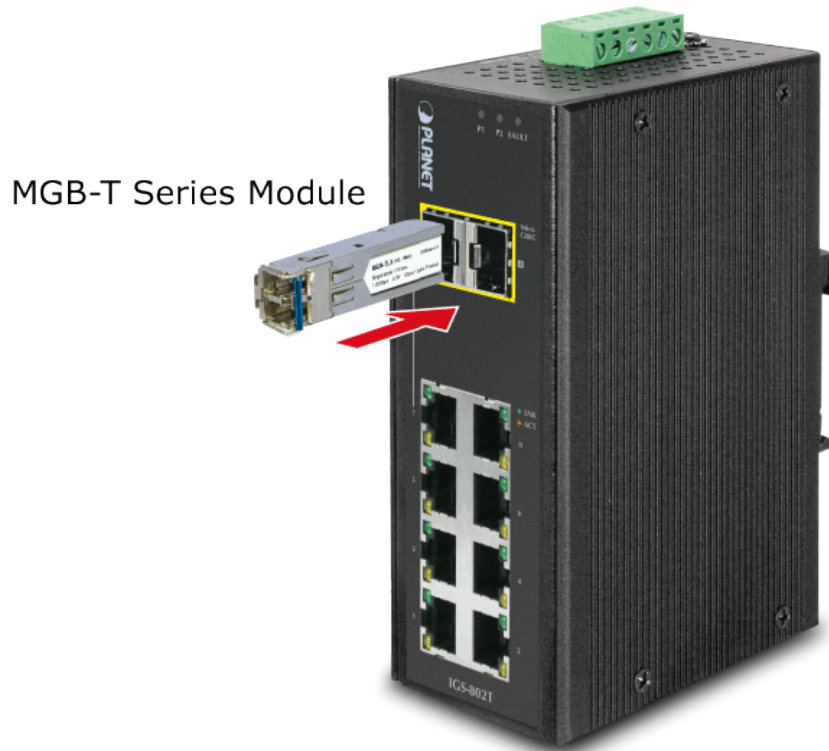
Figure 2-2-4: Plugging in the SFP Transceiver
