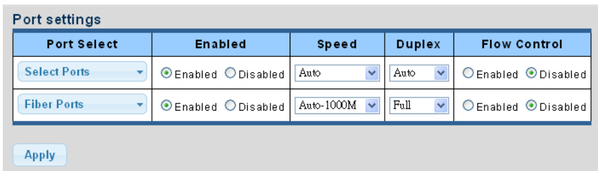
Figure 4-3-1: Port Settings Page Screenshot
