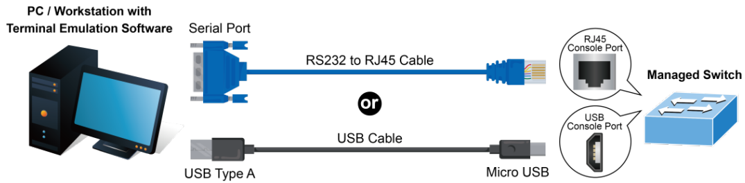
Figure 3-1-1: Console Management
