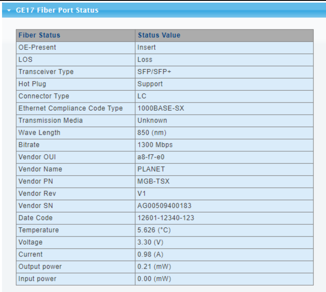
Figure 4-3-21: Fiber Port Status Page Screenshot
