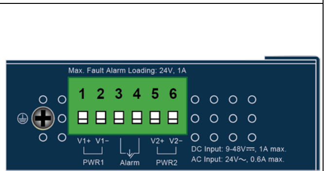
Figure 2-1-4: IGS-4215-16T2S-U Top View
